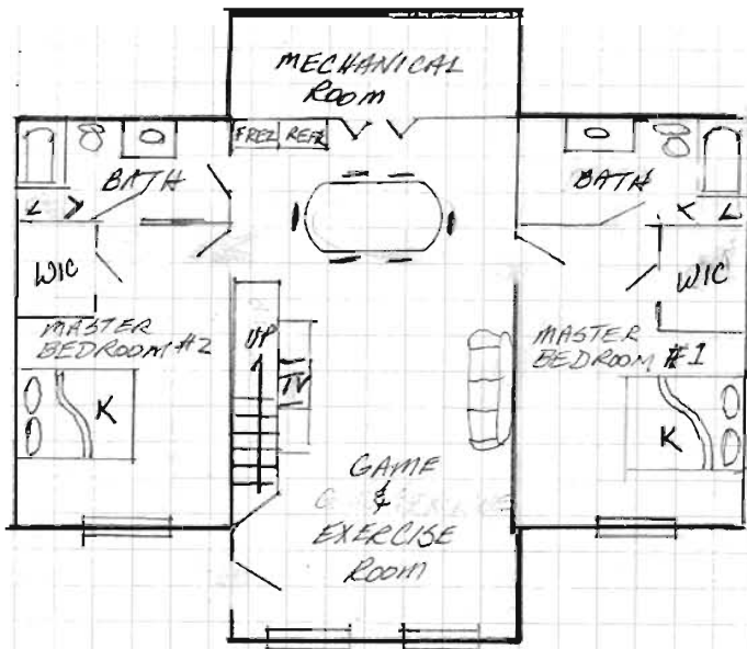
GROUND LEVEL
